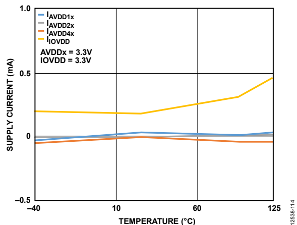
Figure 97. Shutdown Current
